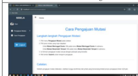
Figure 11. Community dashboard
