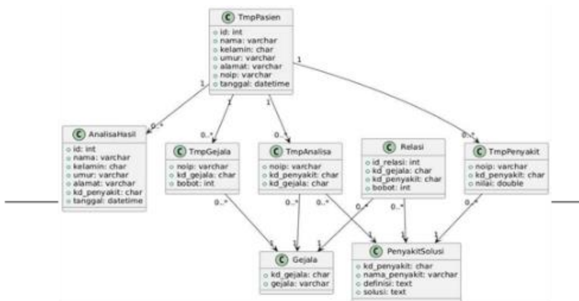
Figure 9. Class Diagram
