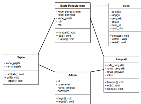
Figure 3. Class Diagram
