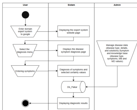
Figure 4. Activity Diagram
