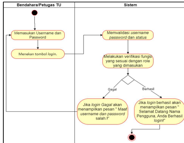
Figure 3. Activity Diagram
