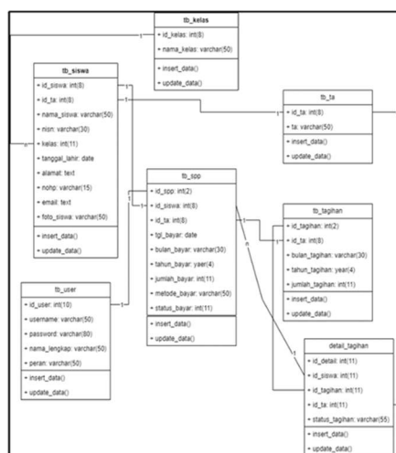
Figure 5. Class Diagram
