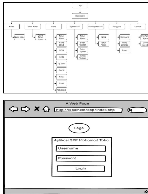
Figure 6. Interface Design
