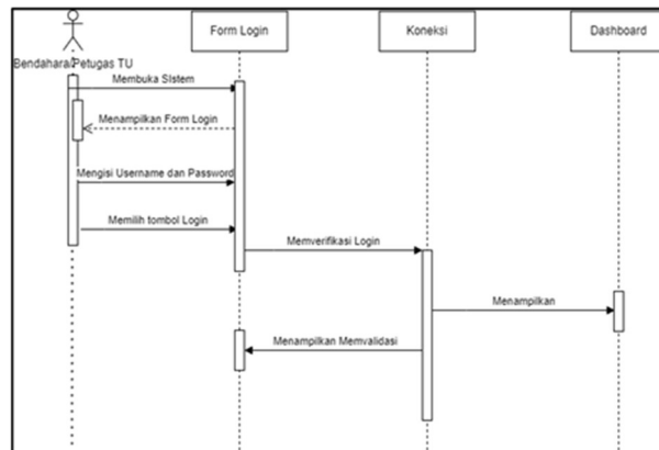
Figure 4. Sequence Diagram
