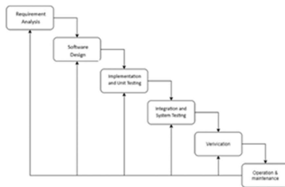
Figure 2. SDLC Stages
