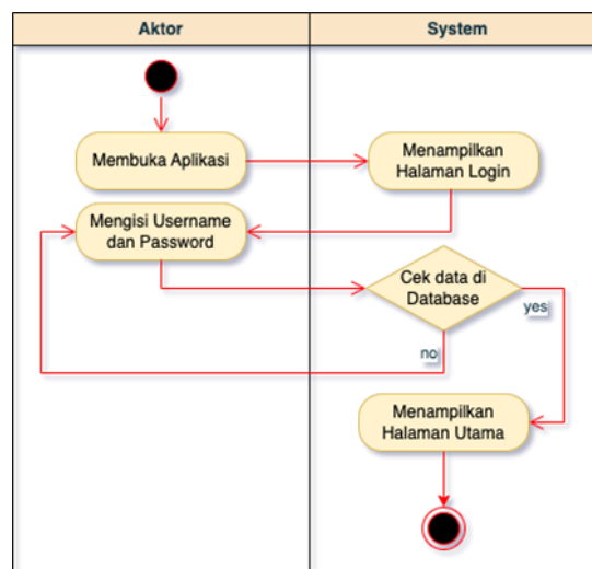
Figure 4. Activity diagram
