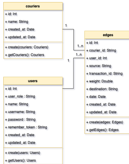
Figure 5. Class Diagram
