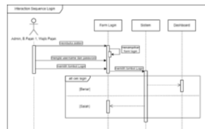
Figure 4. Sequence Diagram
