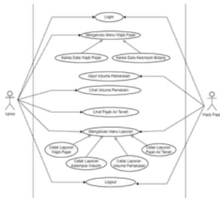
Figure 2. Usecase Diagram
