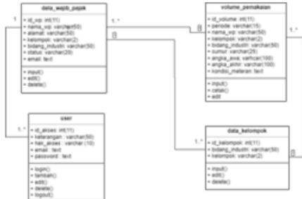
Figure 5. Class Diagram
