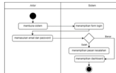
Figure 3. Activity Diagram
