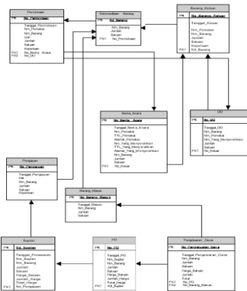
Figure 6. Relational Database
