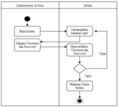
Figure 3. Activity diagram
