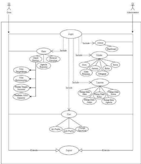
Figure 2. Usecase diagram
