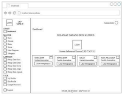
Figure 4. Interface Design
