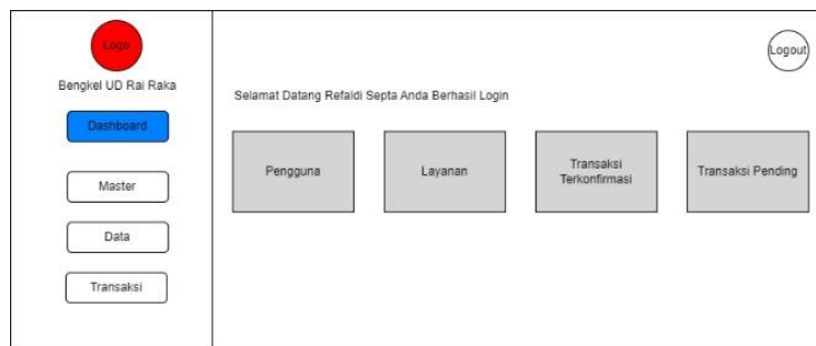
Figure 3. Admin Dashboard
