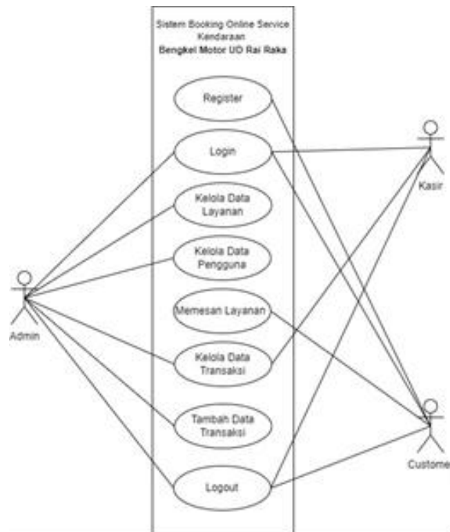
Figure 3. Usecase diagram
