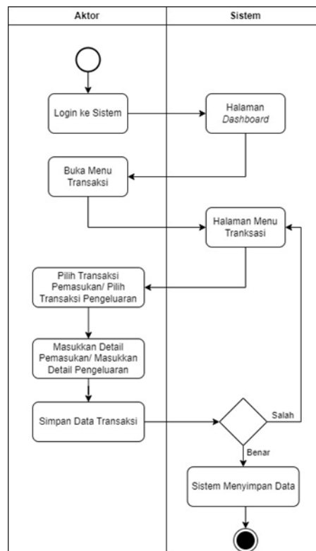
Figure 4. Activity diagram
